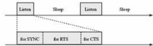
Fig. 1. Periodic listen and sleep in S - MAC[17]
