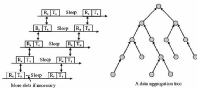
Fig. 2. An aggregation tree in D - MAC[18]
