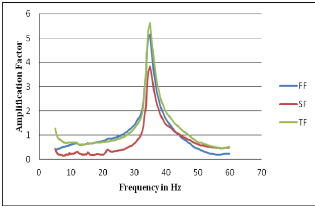
Figure 2.4.A.3 Graph Frequency Vs Amplification Factor
